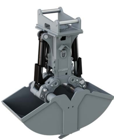
C14TR-60
